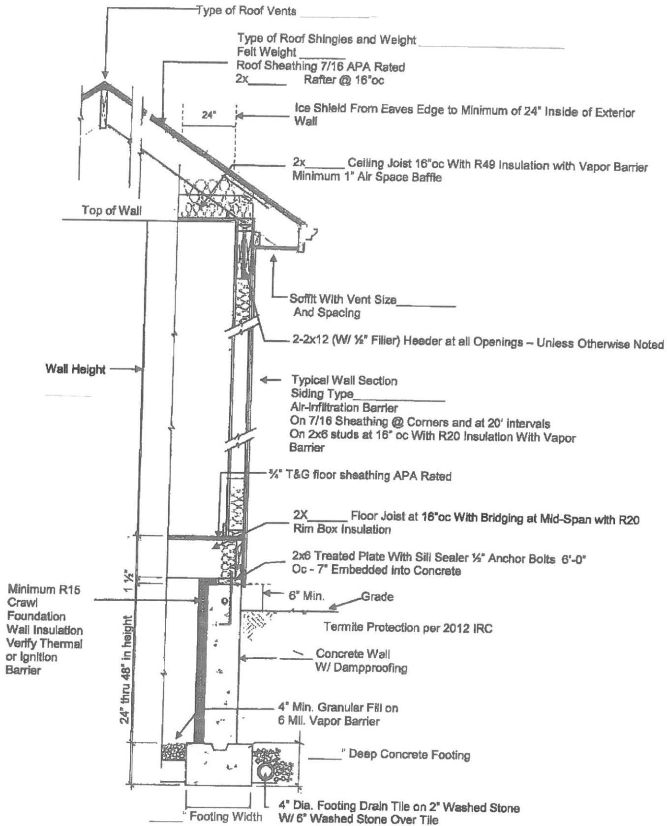
TYPICAL WALL SECTION FOR CRAWL
