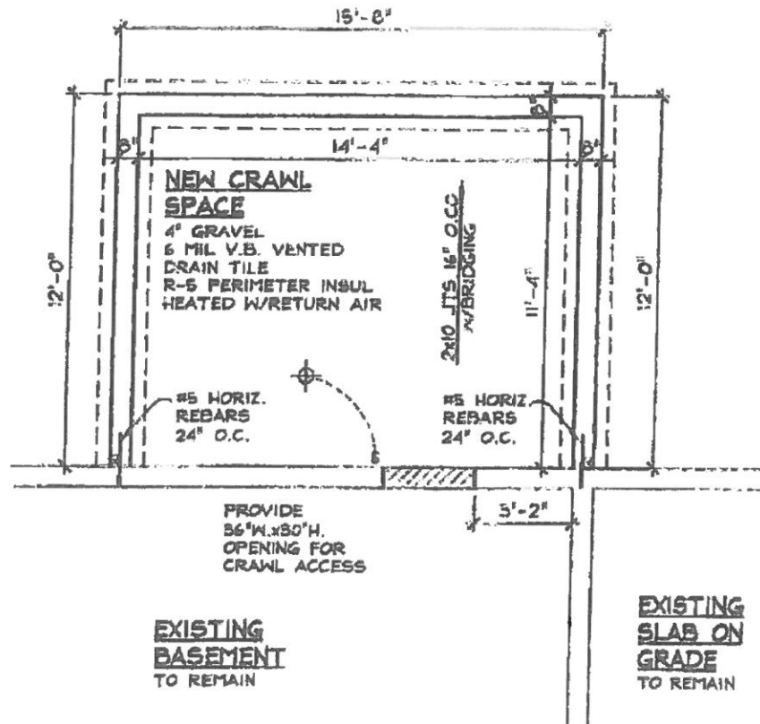
FOUNDATION PLAN
