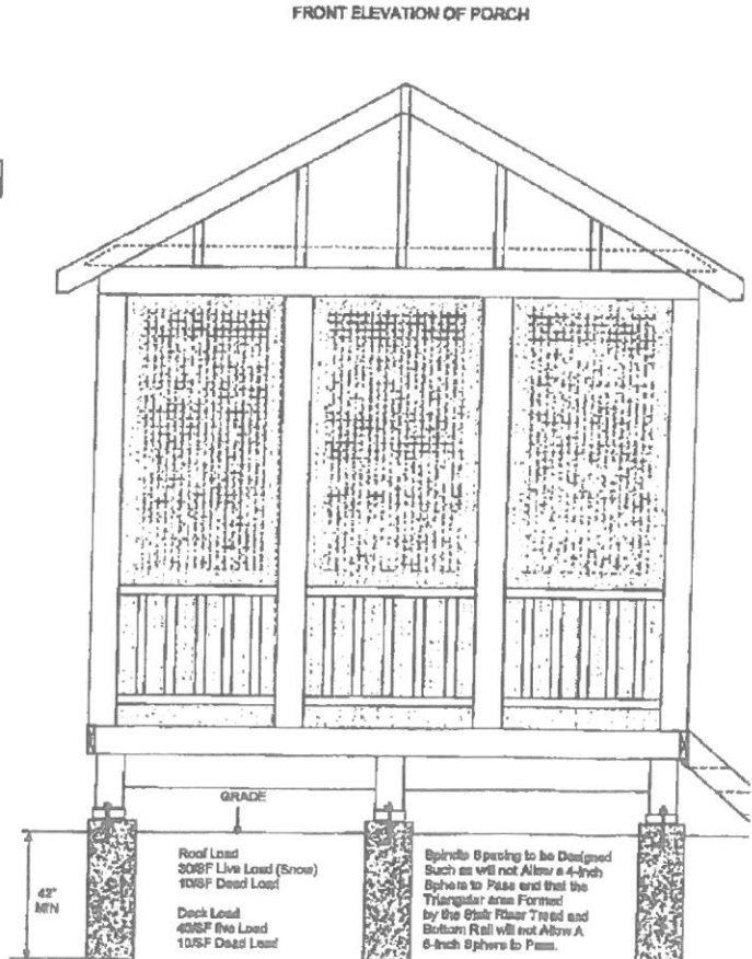
FRONT ELEVATION OF PORCH
