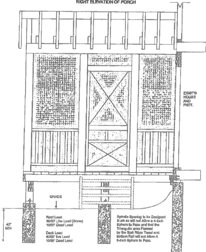
RIGHT ELEVATION OF PORCH
